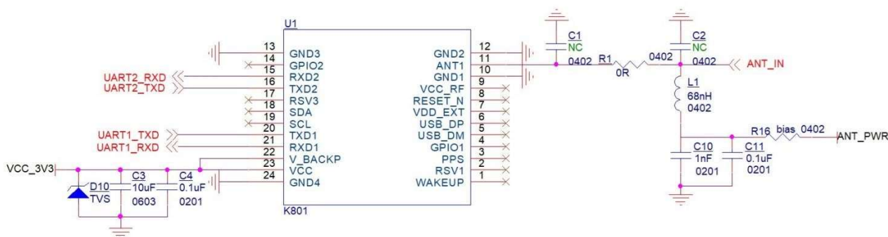
Figure 6. K801S module connection example (active antenna connection mode)/K801S模块连接示例（有源天线连接方式）
