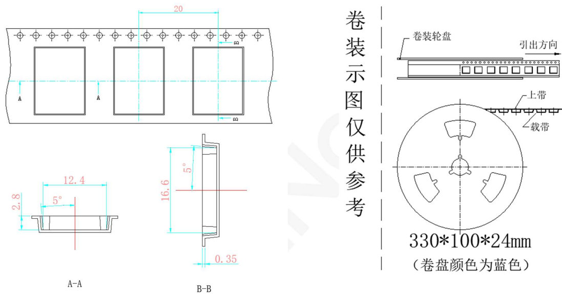
Figure 9. K801S Roll Tape Packing / K801S 卷带包装
