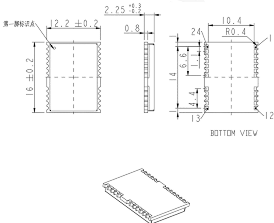
Figure 1. K801S Product Photo / K801S 实物图
