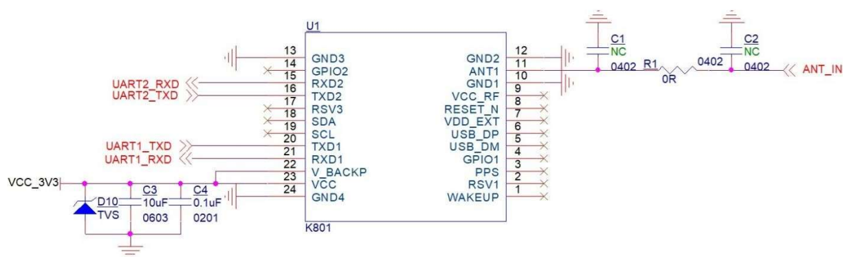
Figure 5. K801S module connection example (passive antenna connection mode)/K801S模块连接示例（无源天线连接方式）
