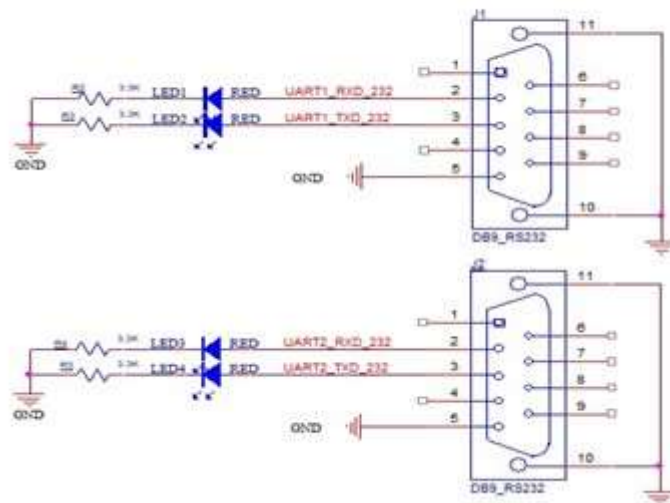
Figure 7. Example of connection between K801S RS232 COM1, 2 and other devices using UART interface / K801S RS232 COM1、2与其他使用UART接口的设备之间的连接示例
