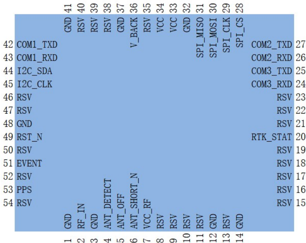
Figure 3. K802A Includes 54-Pin Pad / K802A 包括54连接焊盘
