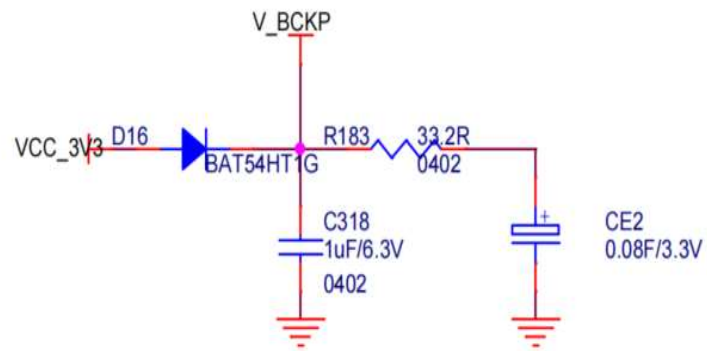
Figure 7. Recommend Design of K802A / K802A 推荐硬件设计
