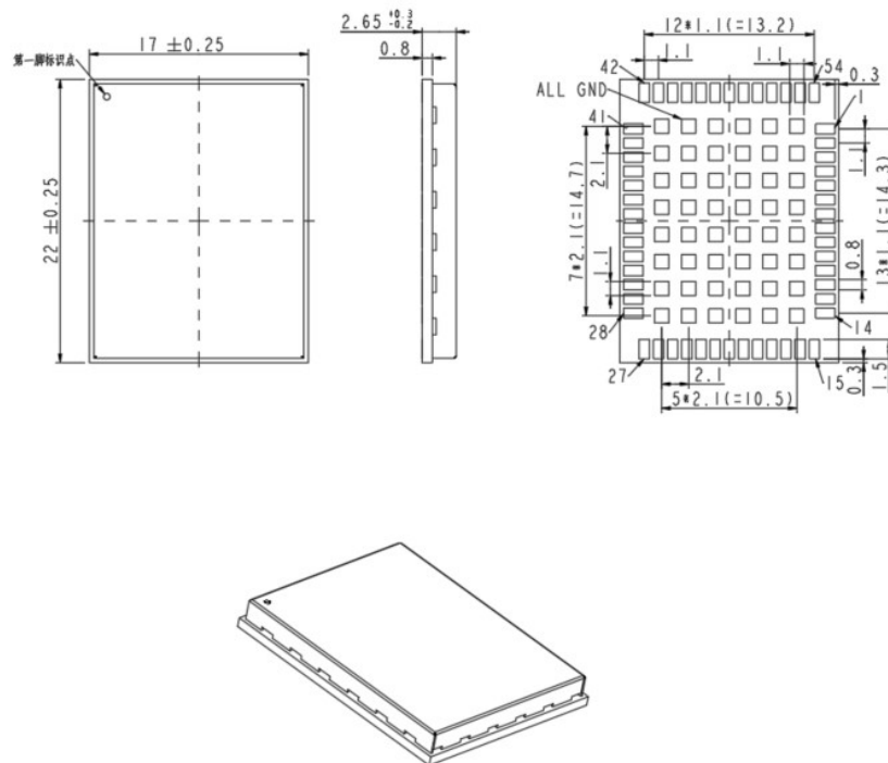
Figure 2. K802A Dimension View / K802A 三视图
