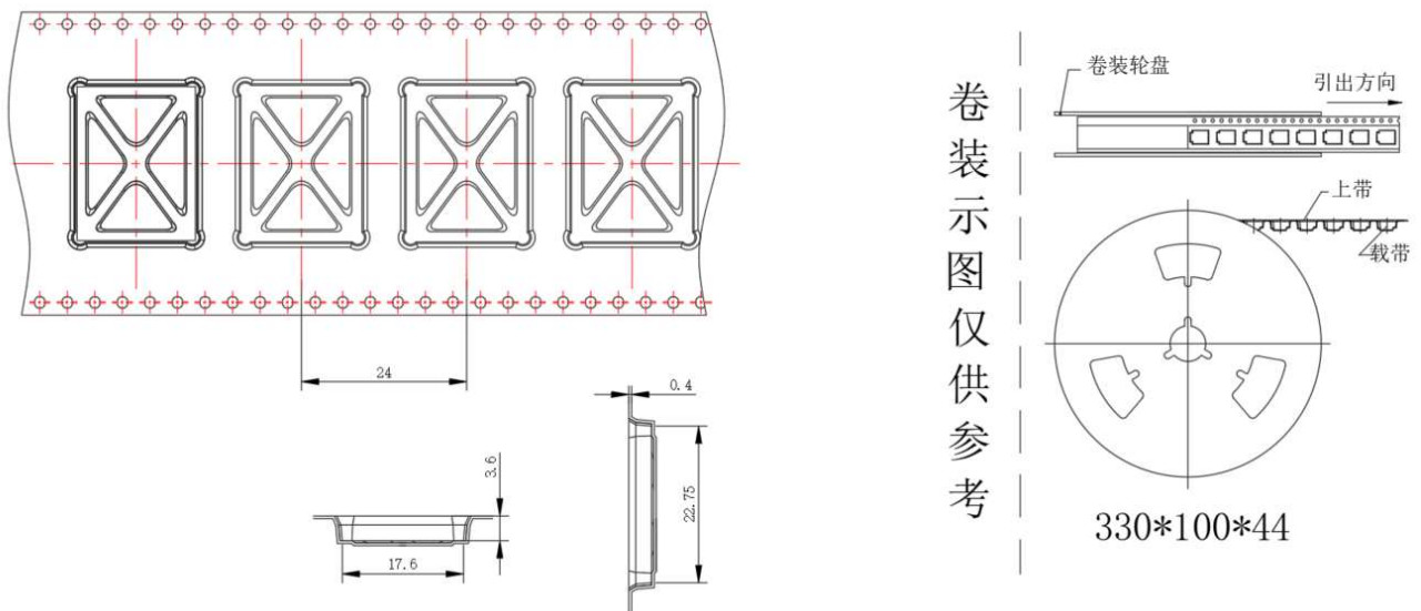
Figure 8. K802A Roll Tape Packing / K802A 卷带包装
