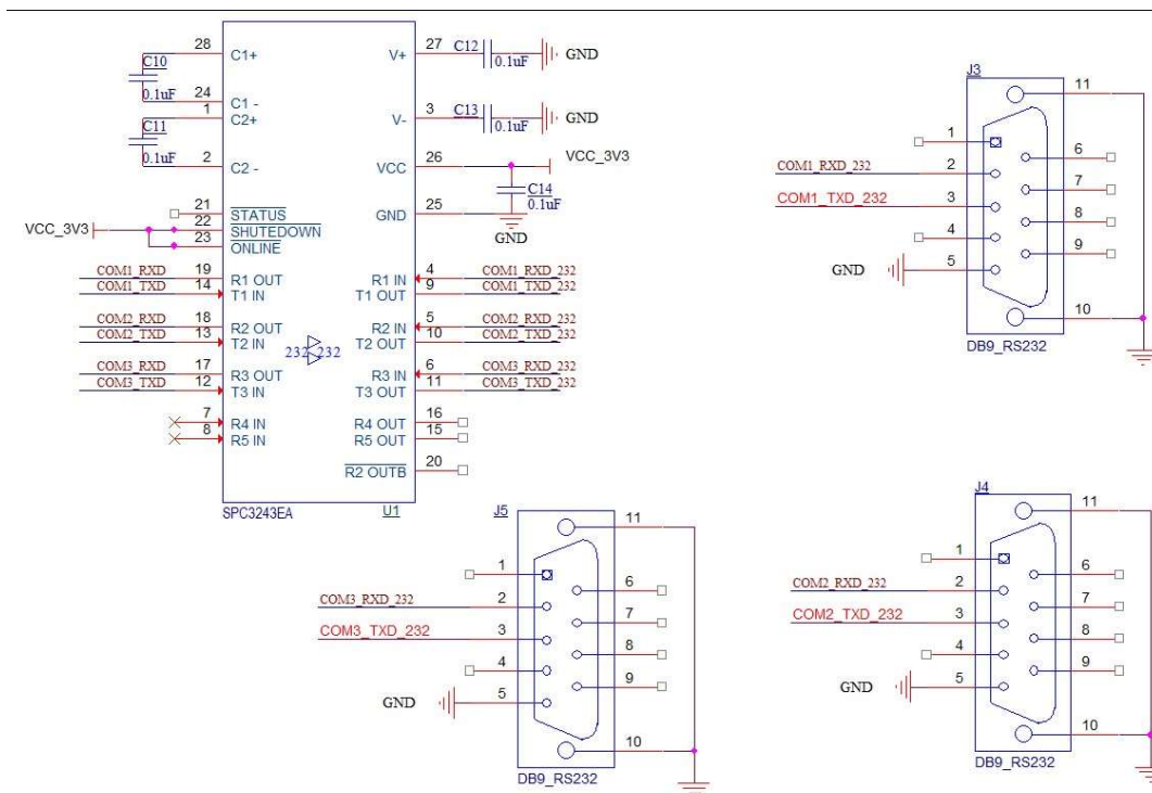
Figure 5. Connections between RS232 COM1, 2, 3 of K802A and Some Other Devices with An UART / K802A RS232 COM1、2、3与其他使用UART接口的设备之间的连接示意
