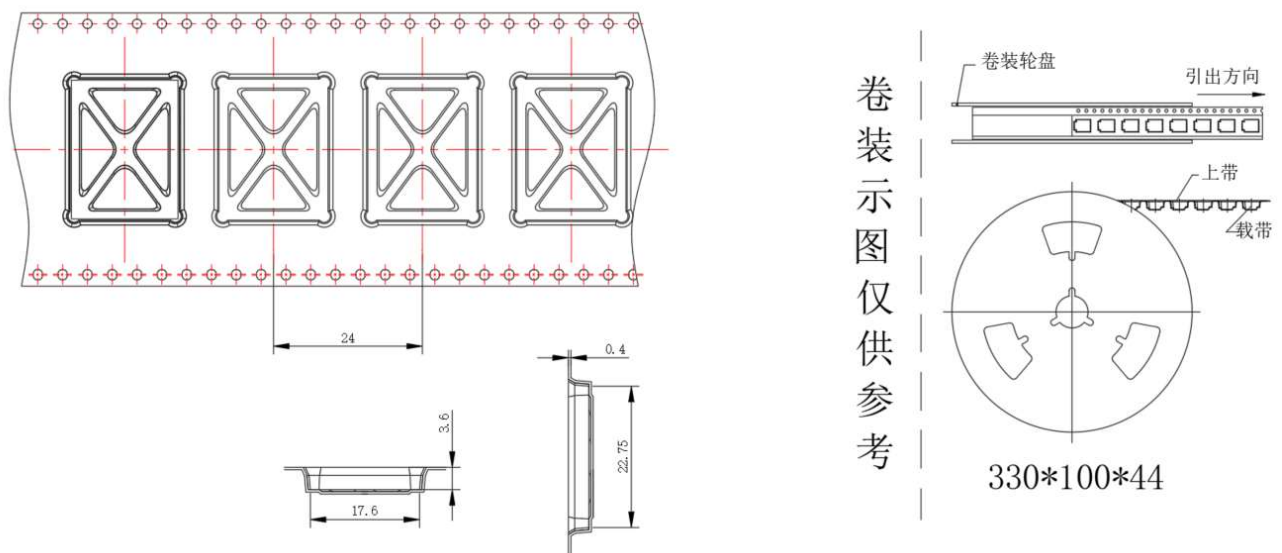
Figure 8. K802F Roll Tape Packing / K802F 卷带包装
