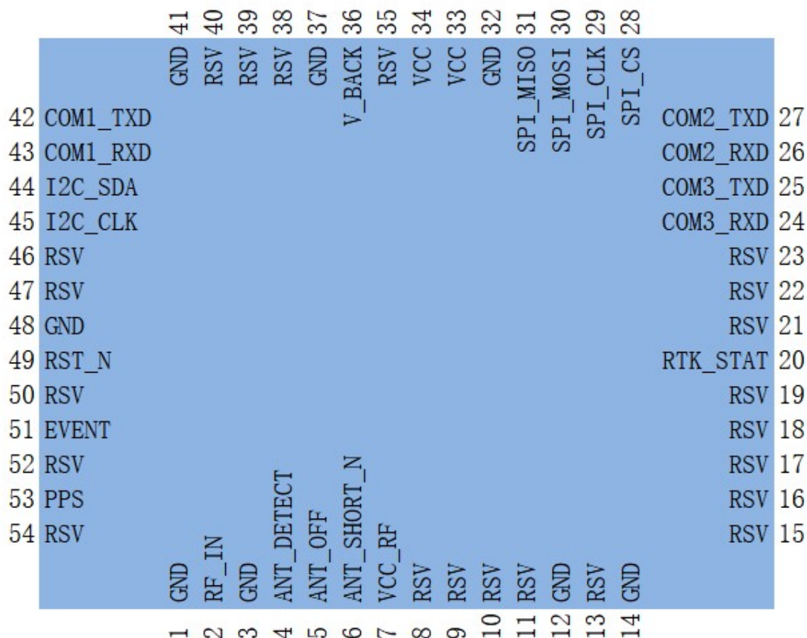
Figure 3. K802F Includes 54-Pin Pad / K802F 包括54连接焊盘
