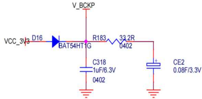
Figure 7. Recommend Design of K802F / K802F 推荐硬件设计
