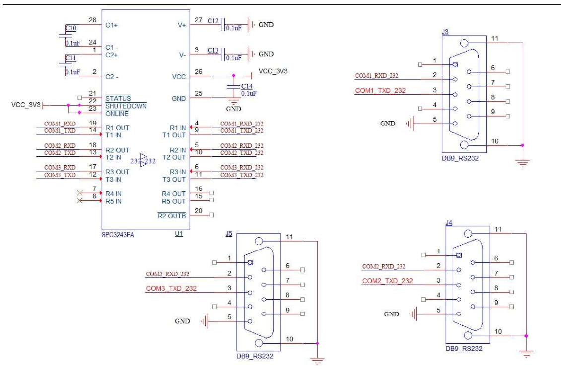
Figure 5. Connections between RS232 COM1, 2, 3 of K802F and Some Other Devices with An UART / K802F RS232 COM1、2、3与其他使用UART接口的设备之间的连接示意
