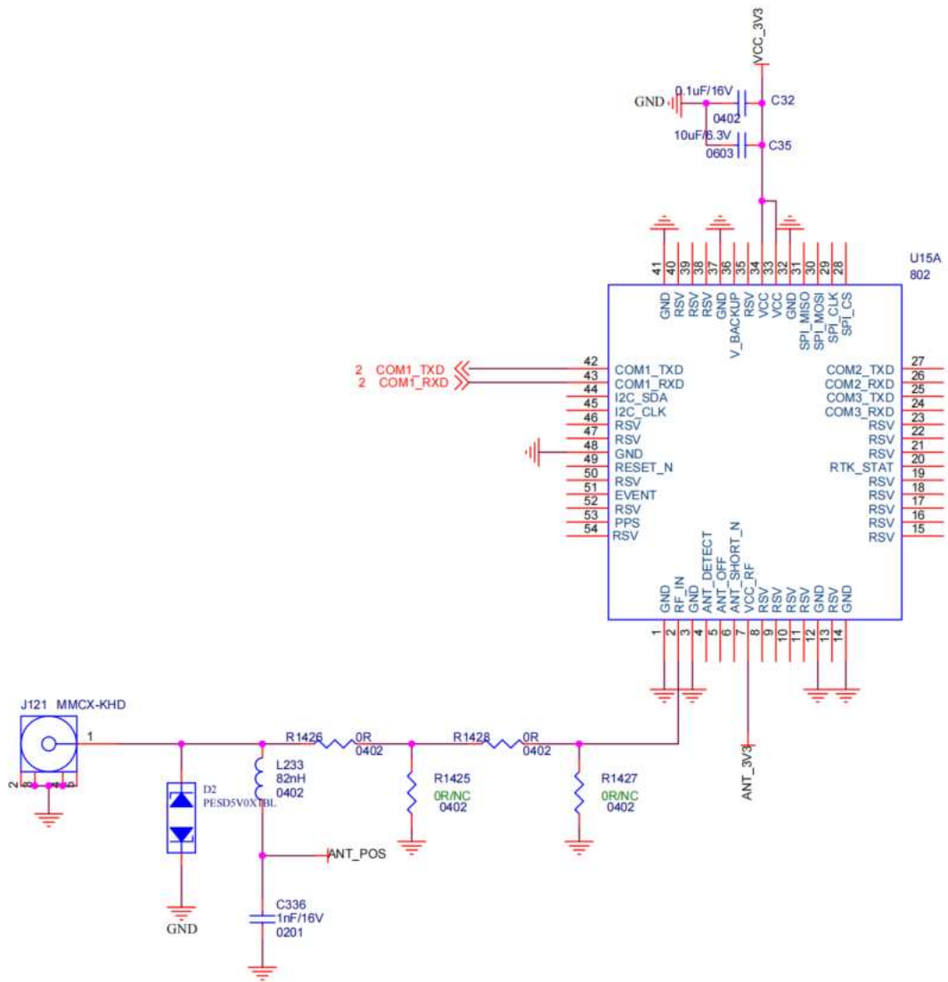
Figure 6. Minimum Hardware Design of K802F / K802F 最小硬件设计
