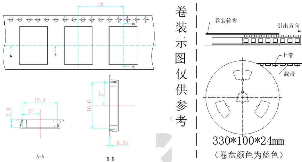
Figure 6. K901 卷带包装
